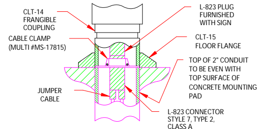
ELECTRICAL CONNECTION DETAIL FIGURE 1
