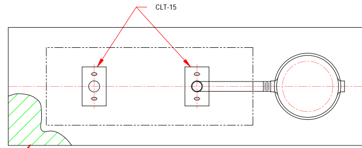
ELECTRICAL CONNECTION DETAIL FIGURE 1
